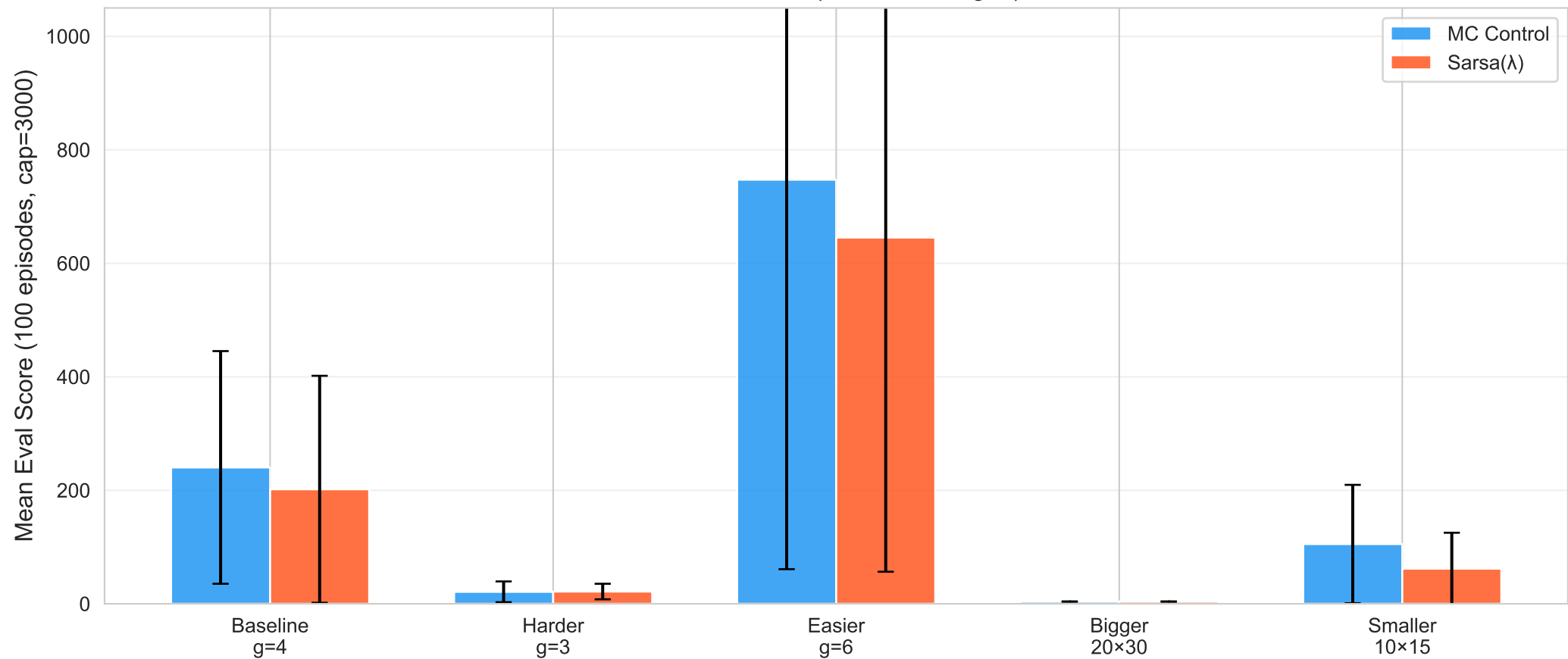
Generalization: Trained on Default (H=15, W=20, g=4), Tested on Variants
