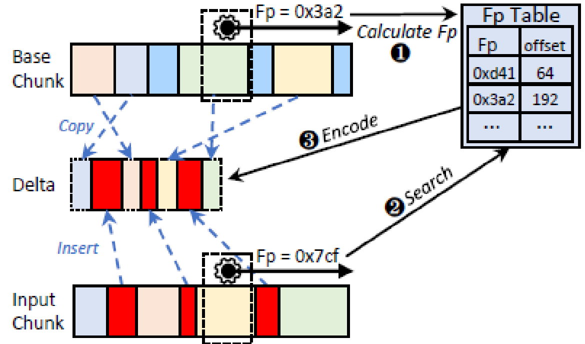
Figure 2: The process of Delta Encoding.
