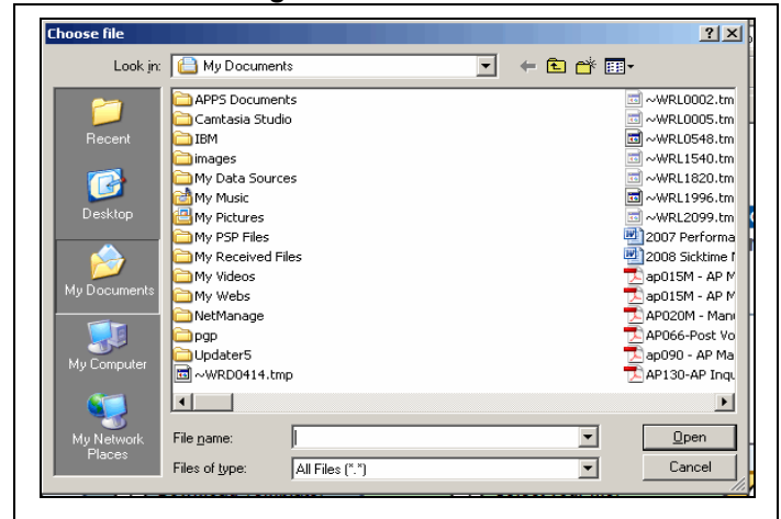
Figure 6 - Choose File
