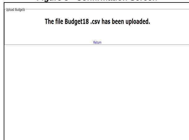
Figure 8 - Confirmation Screen
