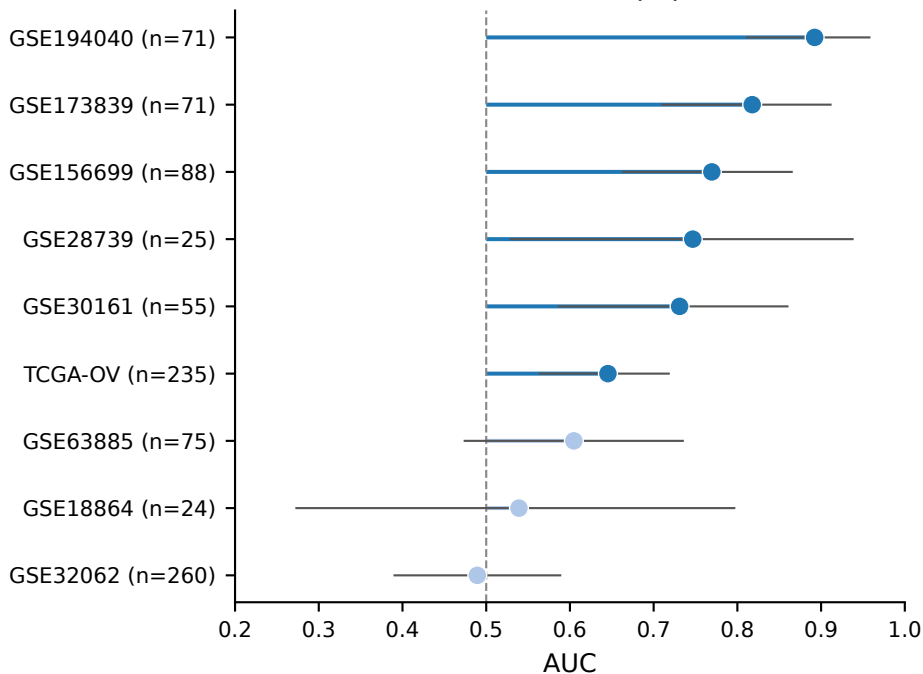
LODO-CV AUC: Lollipop Chart
