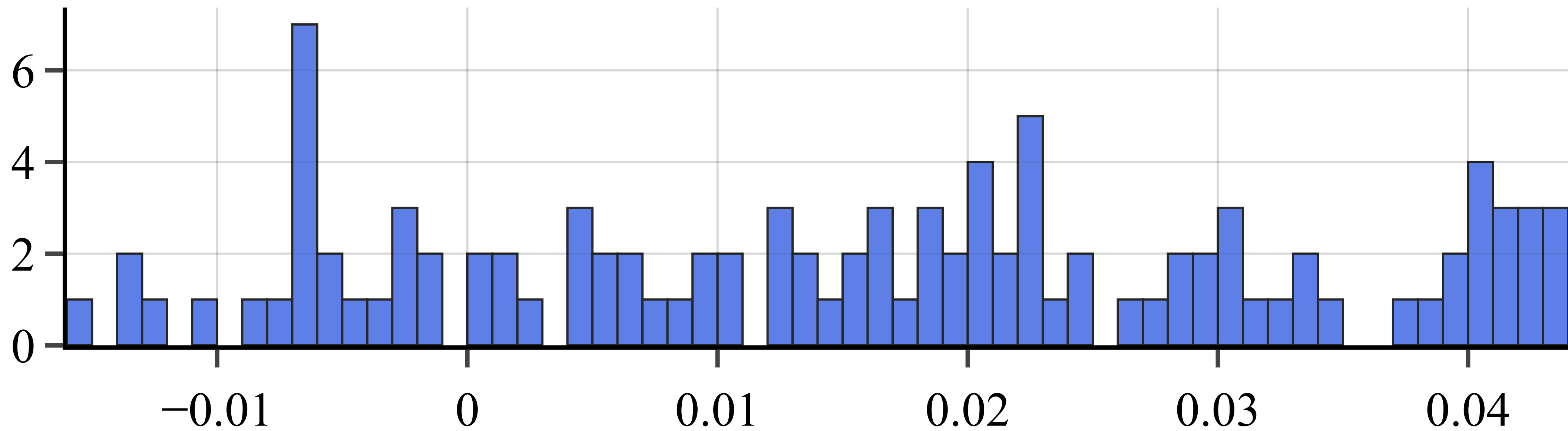
Distance to ray in cluster 11
