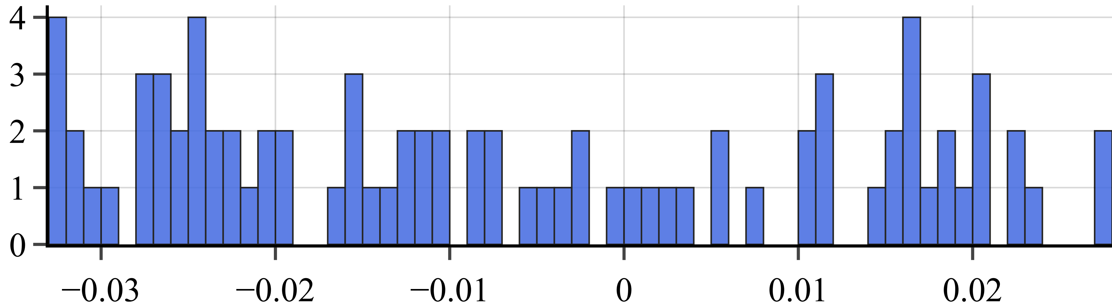
Distance to ray in cluster 14
