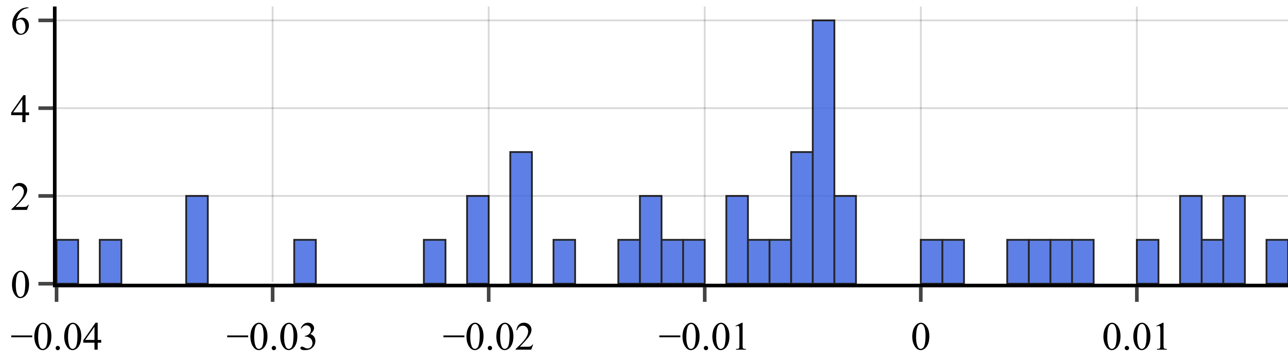
Distance to ray in cluster 18
