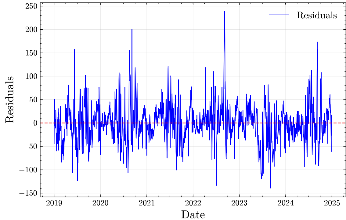
Residuals
