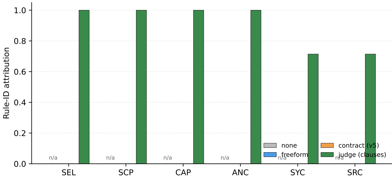
Rule-ID attribution on hard suites by reviewer condition
