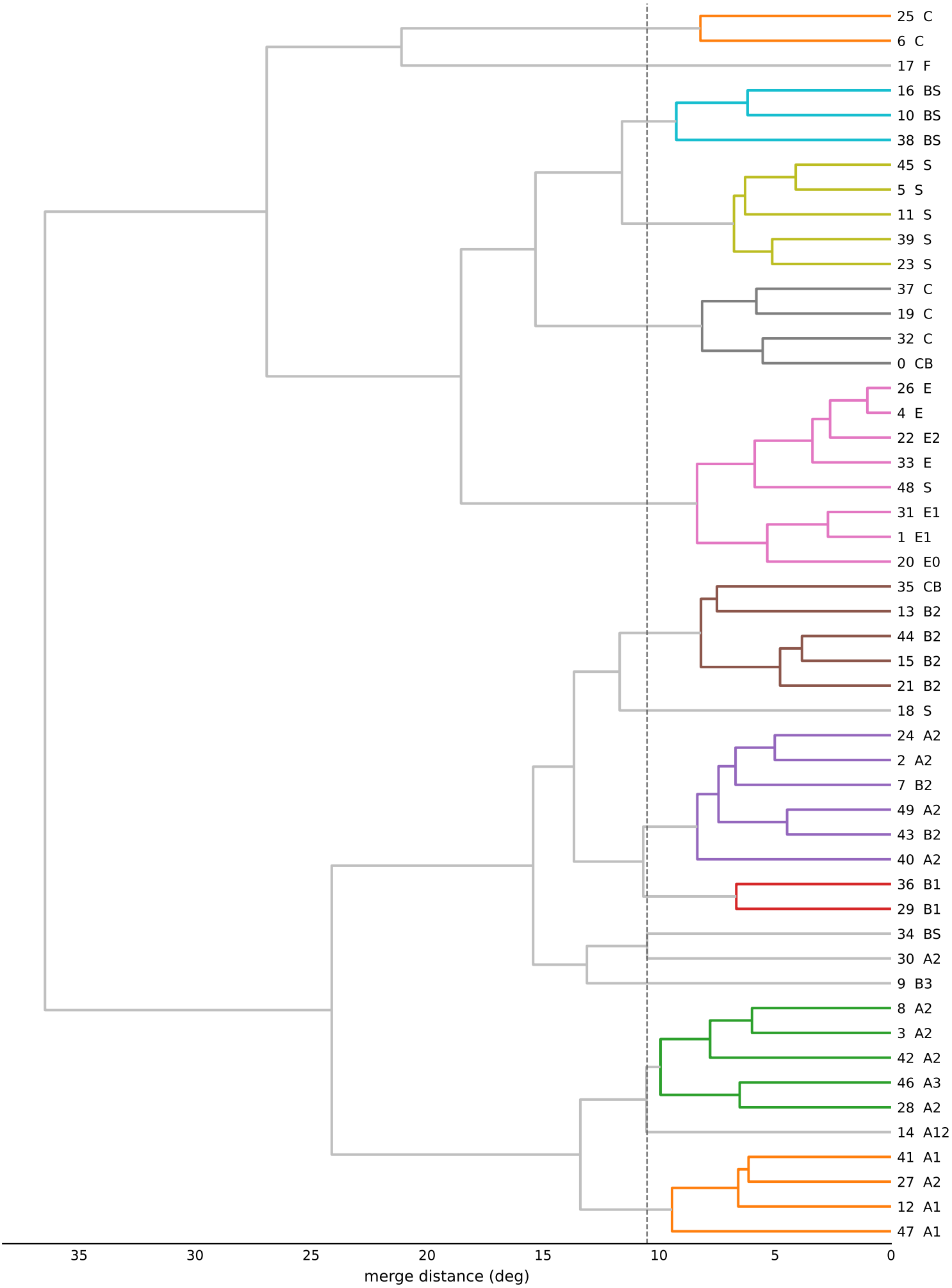
Hierarchical clustering of the 50 centroids (average linkage, cut at 16 groups)
