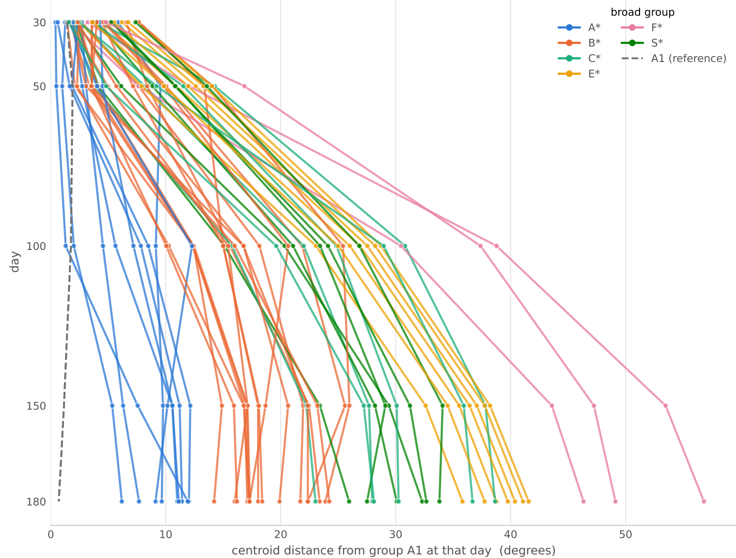
How far each of the 50 clusters sits from group A1, day by day
