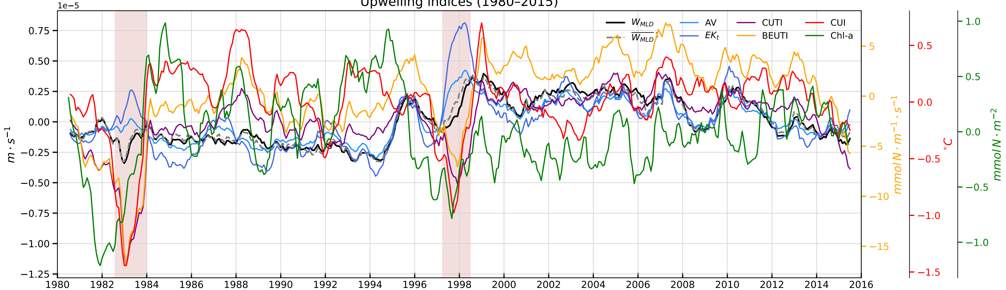
Upwelling indices (1980-2015)
