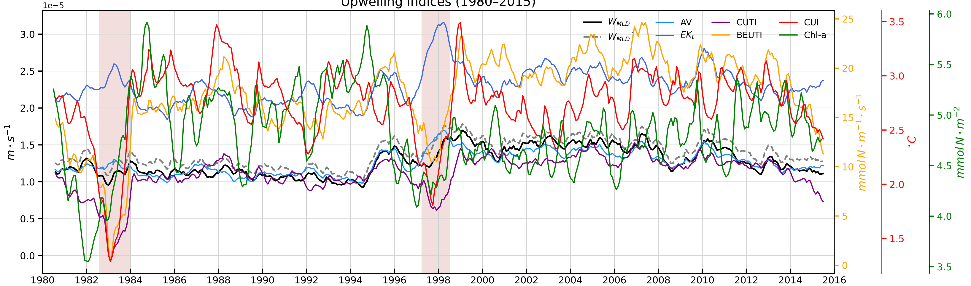
Upwelling indices (1980-2015)
