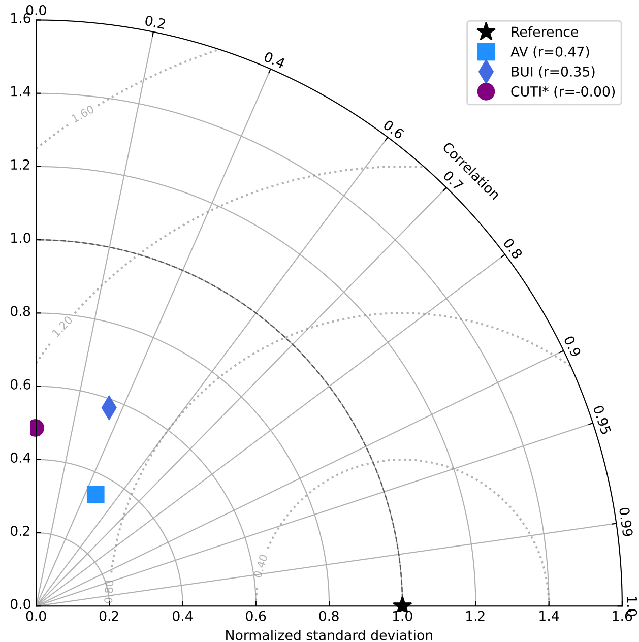
Taylor diagram — UI vs CROCO (each vs its own reference)
