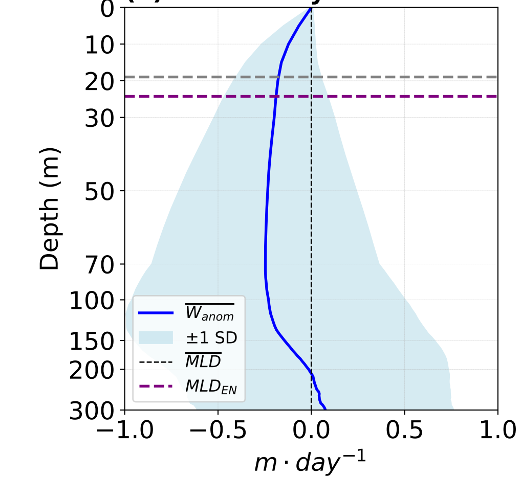
(e) W anomaly 1982-84
