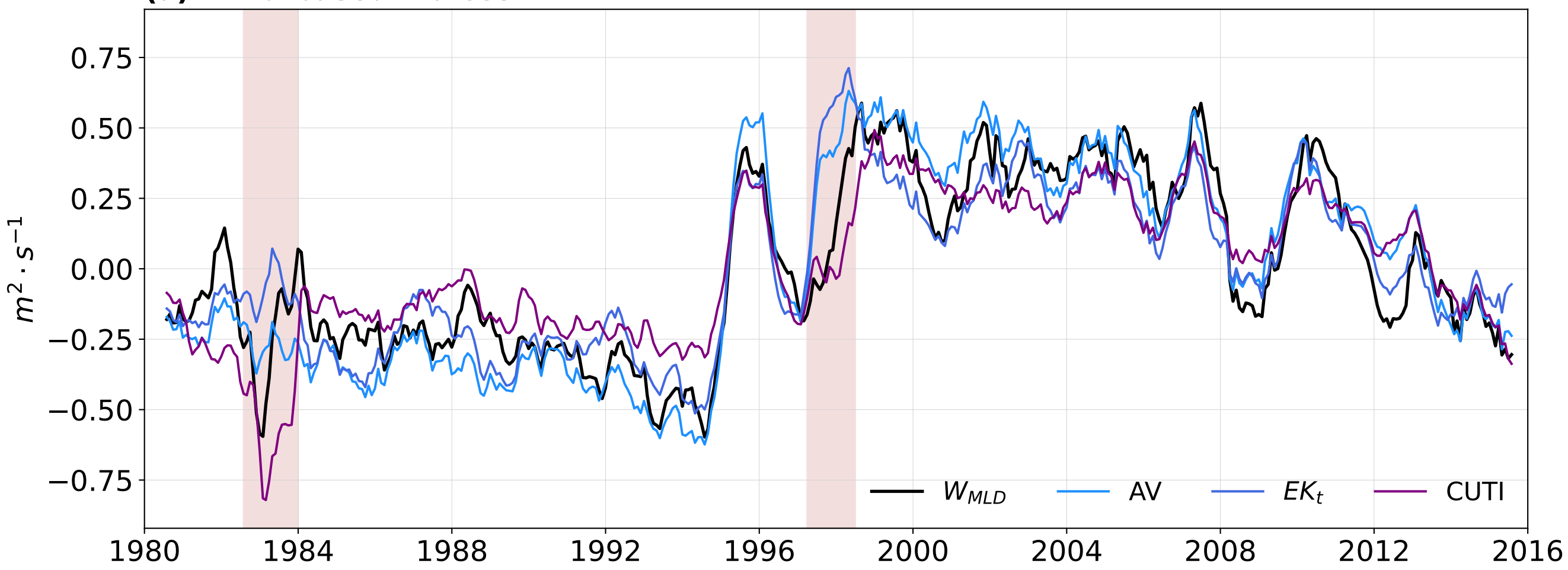
(a) Wind-based indices
