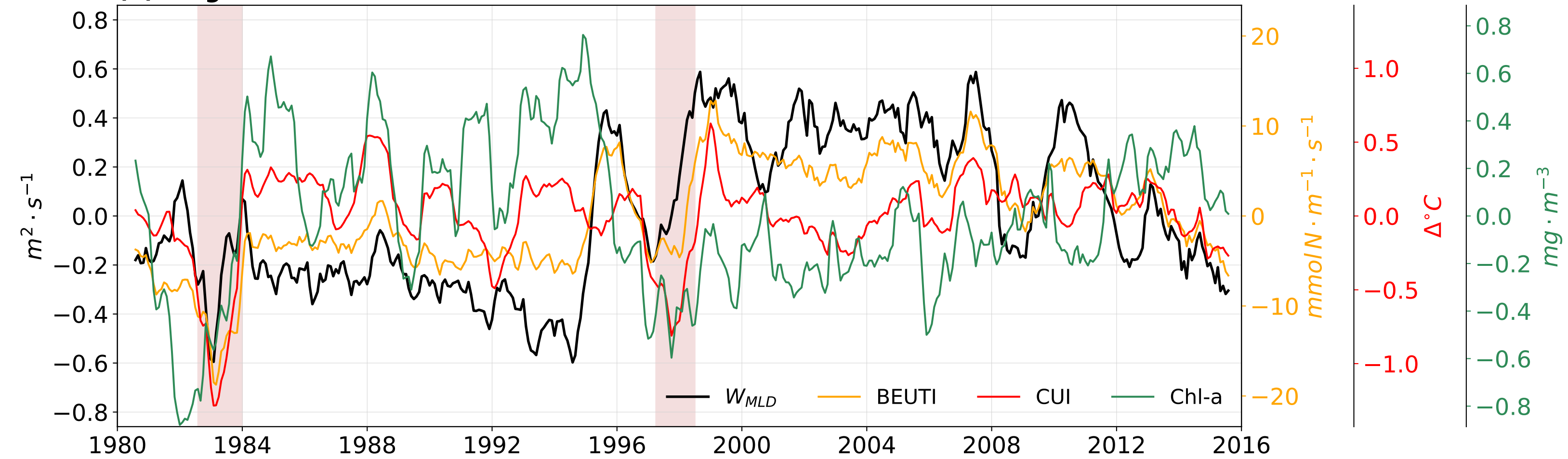
(b) Biogeochemical and SST indices
