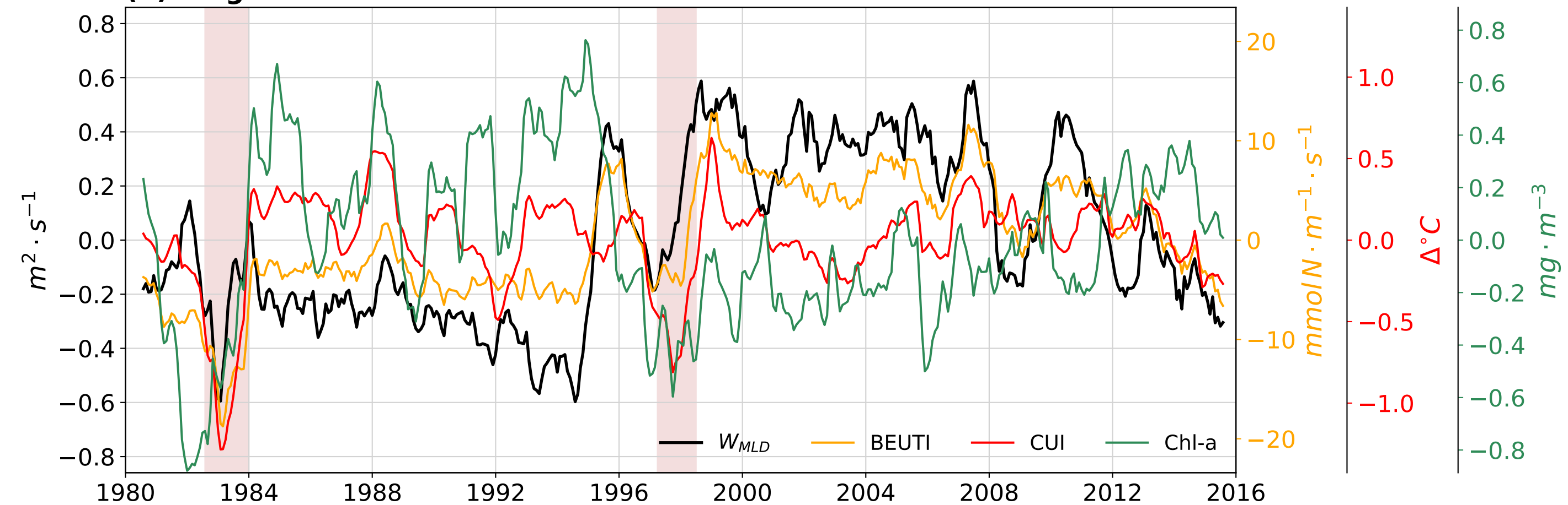
(b) Biogeochemical and SST indices
