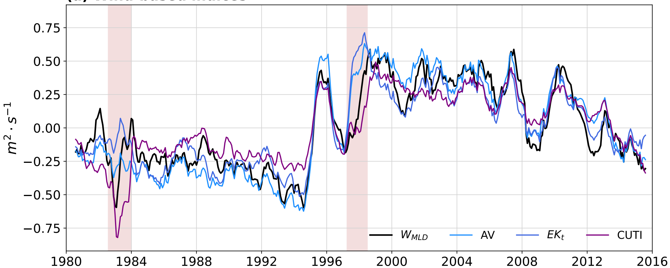
(a) Wind-based indices
