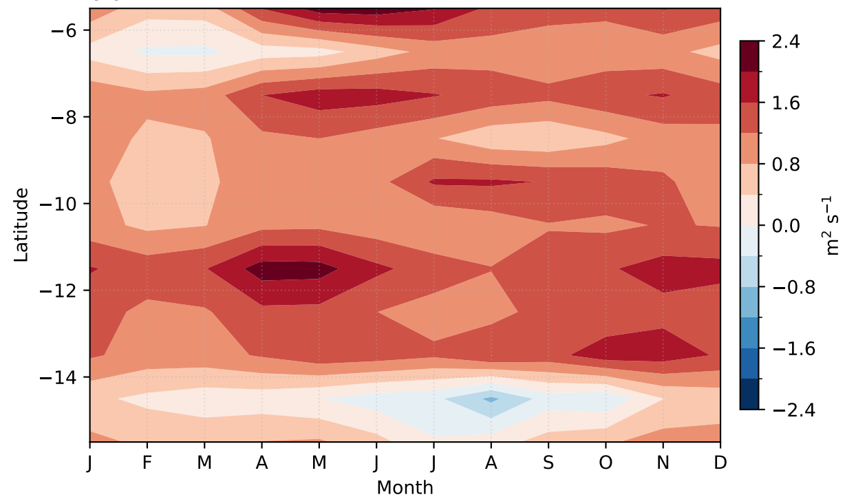
(e) BEUTI
