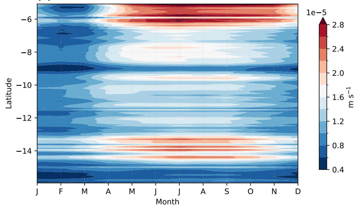
(c) CUTI
