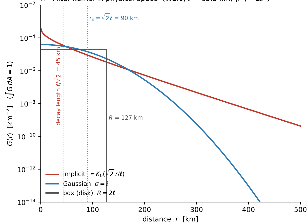
A Filter kernel in physical space ( W2.0 , \ell = 63.5 km, \langle r^2 \rangle = 2\ell^2 )
