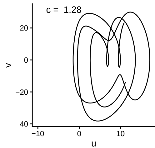
Oscillator trajectory
