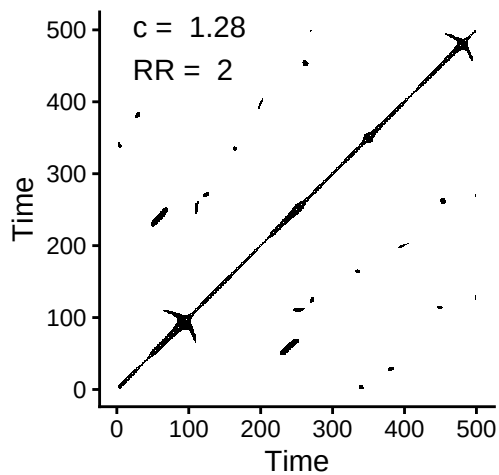
Oscillator RP
