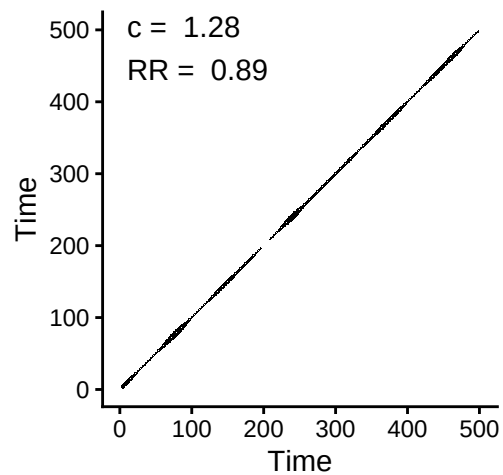
Joint RP
