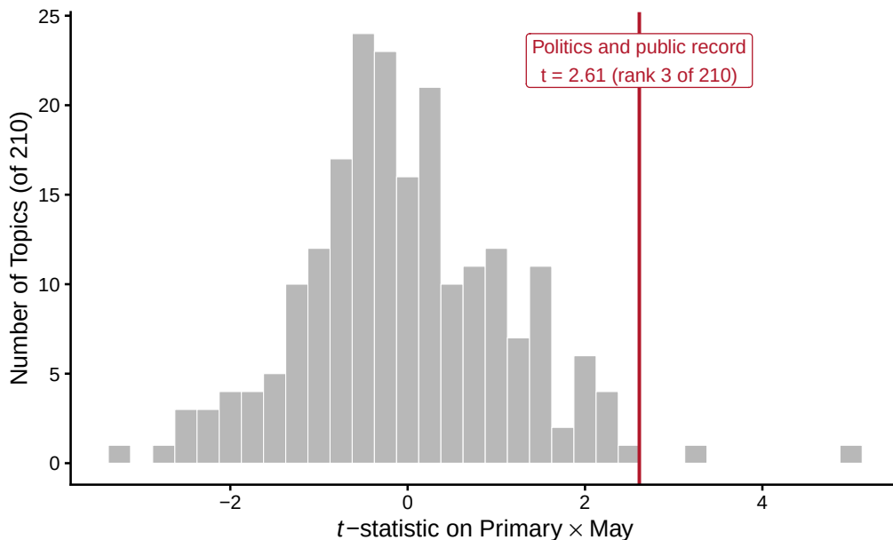
Figure 4: Empirical null distribution. Distribution of t -statistics on Primary \times May across all 210 topic series estimable with the same specification.
