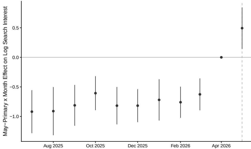
(b) Event-study estimates, reference month April 2026
