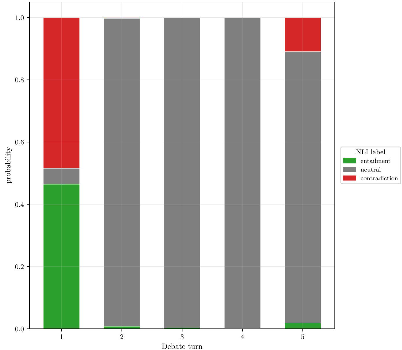
Individual experiment analysis (no stance) — GPT-OSS-120B, faculty manuscript submission, incentive Alignment-Inducing/historical, repeat 5 (b39f482e) NLI self-consistency — junior faculty (no stance)
