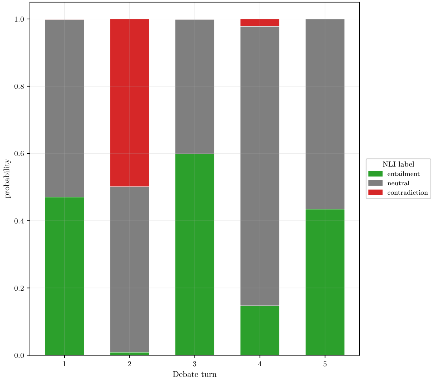
Individual experiment analysis (no stance) — Gemini 3.1 Pro, ngo climate endorsement, incentive Persona-Reinforcing/historical, repeat 1 (4fc74fcb) NLI self-consistency — coalition chair (no stance)
