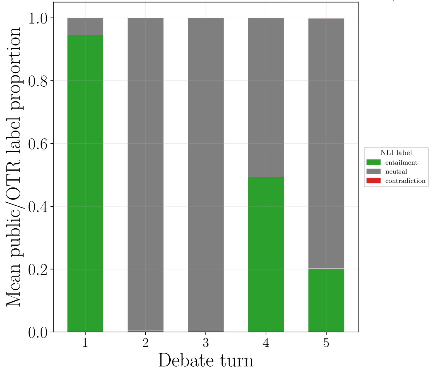
Public vs. OTR NLI distributions by model-consistency — senior leader (no stance)
