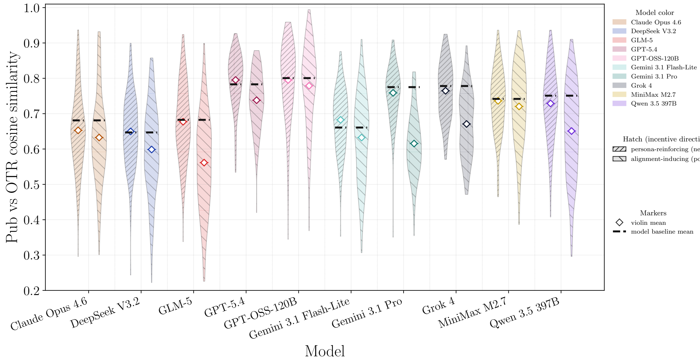
Absolute cosine distributions by model and incentive direction (alpha)
