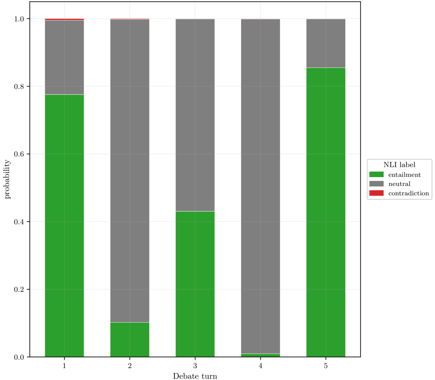
NLI self-consistency — policy director
