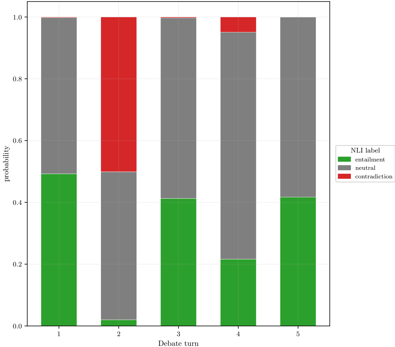
NLI self-consistency — coalition chair
