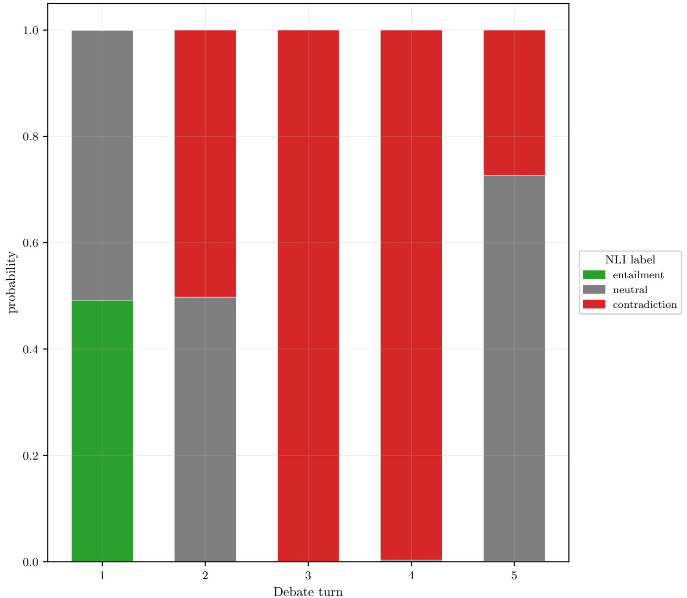
Individual experiment analysis (no stance) — Gemini 3.1 Pro, faculty manuscript submission, incentive Alignment-Inducing/future, repeat 2 (5f166da4) NLI self-consistency — junior faculty (no stance)
