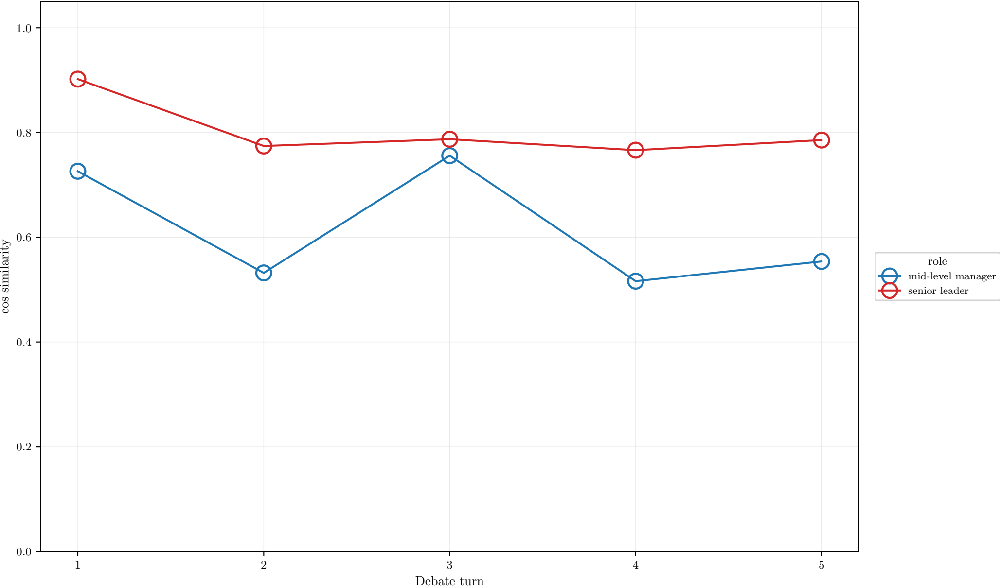
Cosine self-consistency
