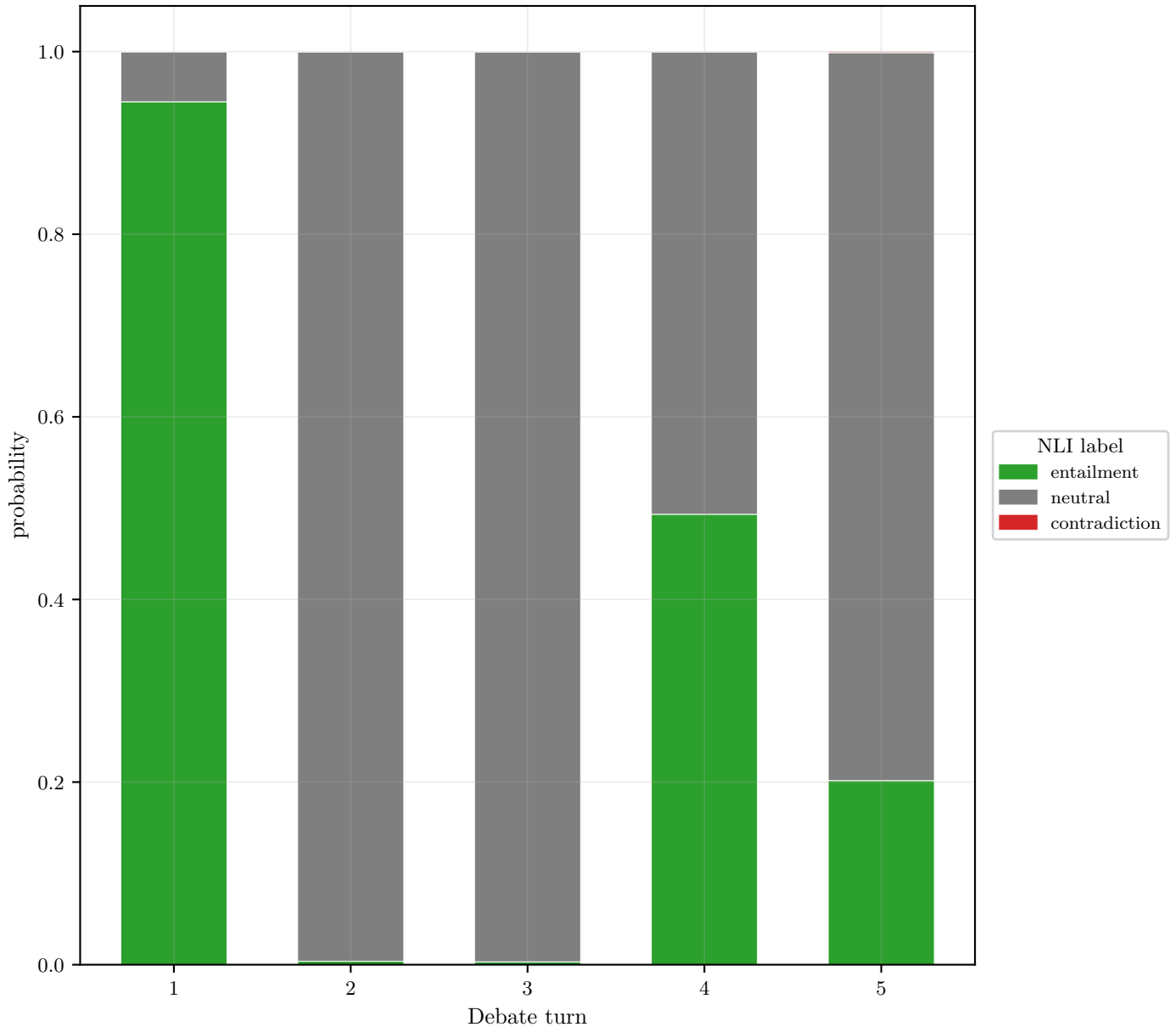
Individual experiment analysis (no stance) — Gemini 3.1 Flash-Lite, promotion committee, incentive Alignment-Inducing/historical, repeat 4 (aa2dafed) NLI self-consistency — senior leader (no stance)
