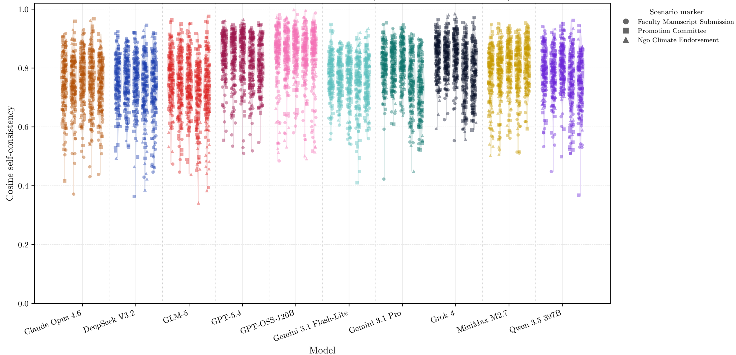
Cosine distributions by model and incentive combo (all scenarios, repeats, rounds)
