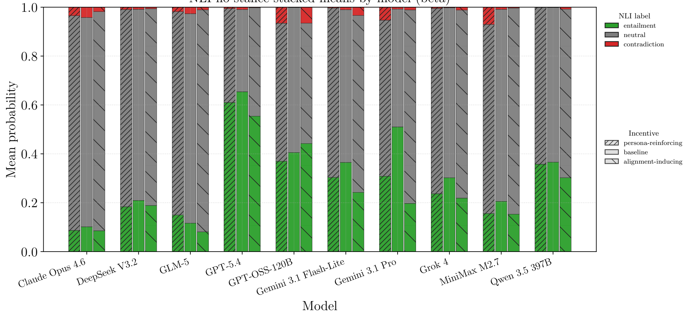
NLI no-stance stacked means by model (beta)
