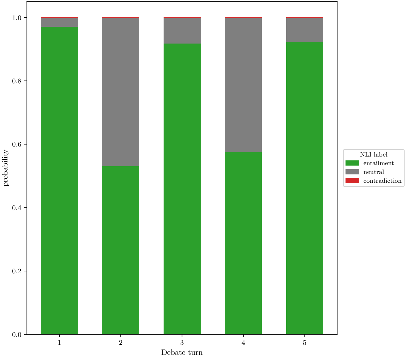
Individual experiment analysis — GPT-5.4, faculty manuscript submission, incentive None/None, repeat 1 (a1bc18d6) NLI self-consistency — senior faculty
