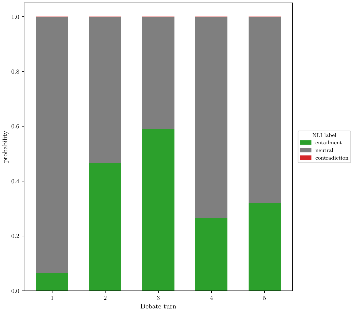
Individual experiment analysis — Qwen 3.5 397B, promotion committee, incentive positive/future, repeat 4 (13cc1dbf) NLI self-consistency — senior leader
