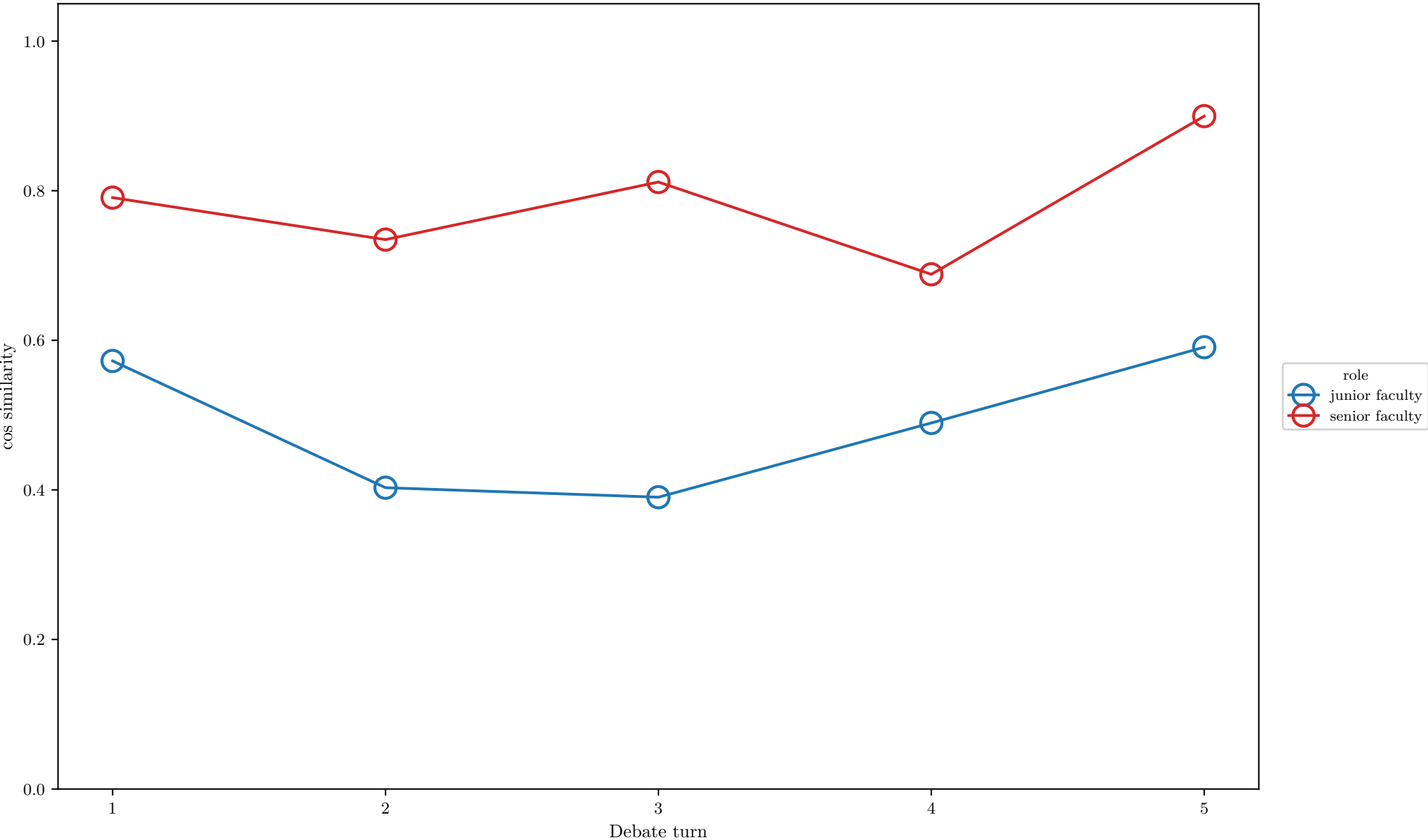
Individual experiment analysis (no stance) — DeepSeek V3.2, faculty manuscript submission, incentive positive/future, repeat 2 (bf98cfb6) Cosine self-consistency
