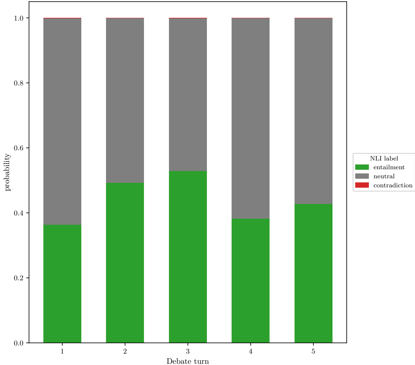
NLI self-consistency — senior leader
