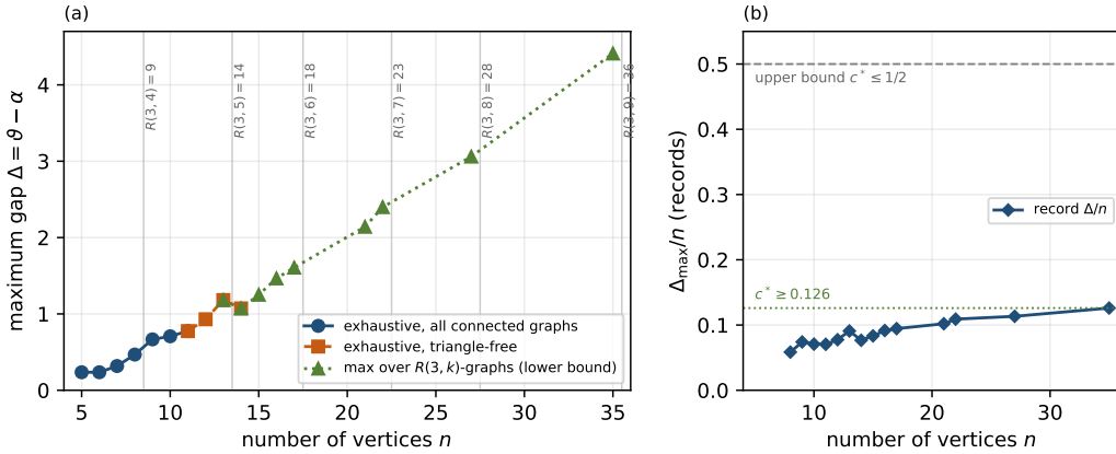
Figure 3: (a) Maximum contextuality gap versus number of vertices: exhaustive over all connected graphs ( n \leq 11 ), exhaustive over triangle-free graphs ( n \leq 14 ), and lower bounds from the complete catalogues of R(3, k) -graphs. Vertical lines mark the Ramsey numbers R(3, k) , where \alpha is forced up by one for triangle-free graphs. (b) Gap per vertex of the record graphs, with the bounds 0.126 \leq c^* \leq \frac{1}{2} of Proposition 3; the sequence is still increasing at n = 35 .
