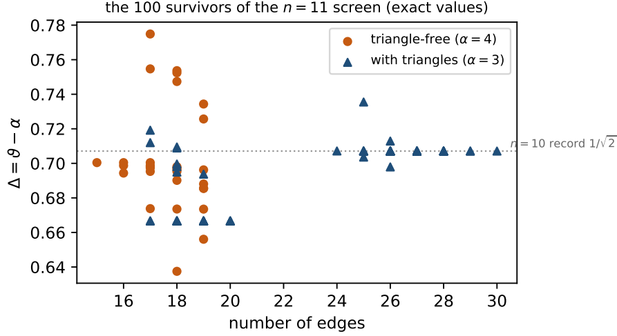
Figure 2: The 100 graphs on eleven vertices whose certified bound survived the screen (threshold 1/\sqrt{2} ), with their exact gaps: the sparse triangle-free family ( \alpha = 4 ) and the dense family ( \alpha = 3 , containing the Wagner graph).
