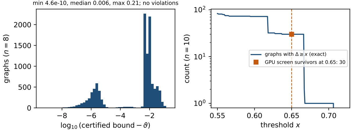
Figure 4: Validation of the GPU screen. (a) Certified upper bound minus exact \vartheta for all connected graphs on eight vertices, without pruning. (b) At n = 10 : number of graphs with \Delta \geq x from the exact run, and the number of survivors of the screen at threshold 0.65, which coincides with the exact count.
