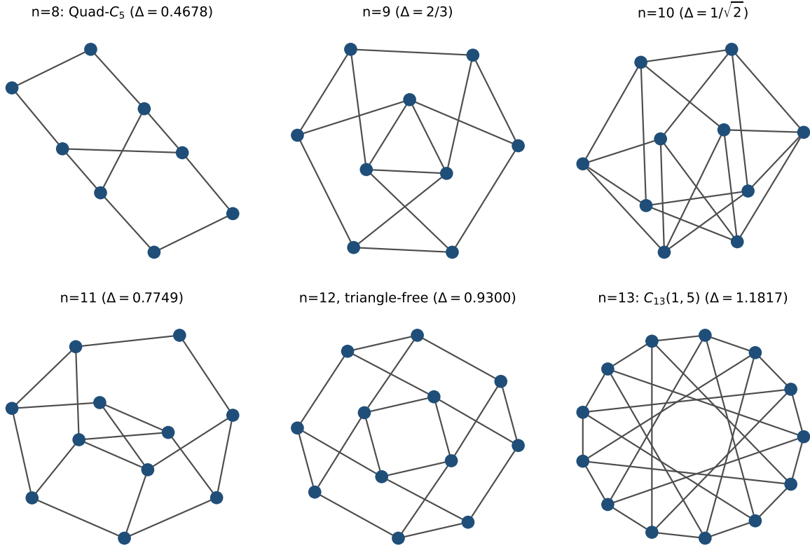
Figure 1: Record graphs. Top: the exhaustive maximizers for n = 8 (Quad- C_5 , [9]), n = 9 and n = 10 . Bottom: the exhaustive maximizer for n = 11 , the triangle-free maximizer for n = 12 , and the triangle-free maximizer for n = 13 , which is the circulant Ramsey graph C_{13}(1, 5) .
