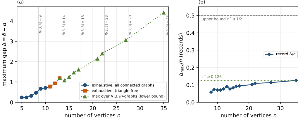
Figure 3: (a) Maximum contextuality gap versus number of vertices: exhaustive over all connected graphs ( n \leq 11 ), exhaustive over triangle-free graphs ( n \leq 13 ), and lower bounds from the complete catalogues of R(3, k) -graphs. Vertical lines mark the Ramsey numbers R(3, k) , where \alpha is forced up by one for triangle-free graphs. (b) Gap per vertex of the record graphs, with the bounds 0.126 \leq c^* \leq \frac{1}{2} of Proposition 3; the sequence is still increasing at n = 35 .
