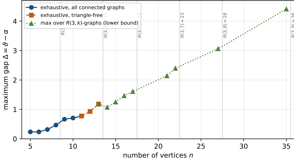
Figure 2: Maximum contextuality gap versus number of vertices: exhaustive over all connected graphs ( n \leq 11 ), exhaustive over triangle-free graphs ( n \leq 13 ), and lower bounds from the complete catalogues of R(3, k) -graphs. Vertical lines mark the Ramsey numbers R(3, k) , where \alpha is forced up by one for triangle-free graphs.
