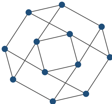
n=12 , triangle-free ( \Delta = 0.9300 )
