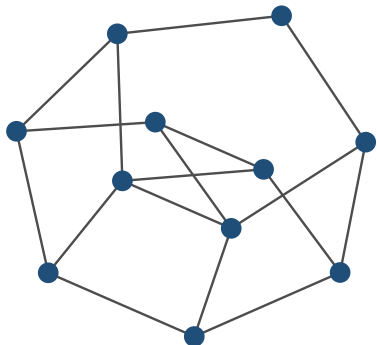
n=11 ( \Delta = 0.7749 )
