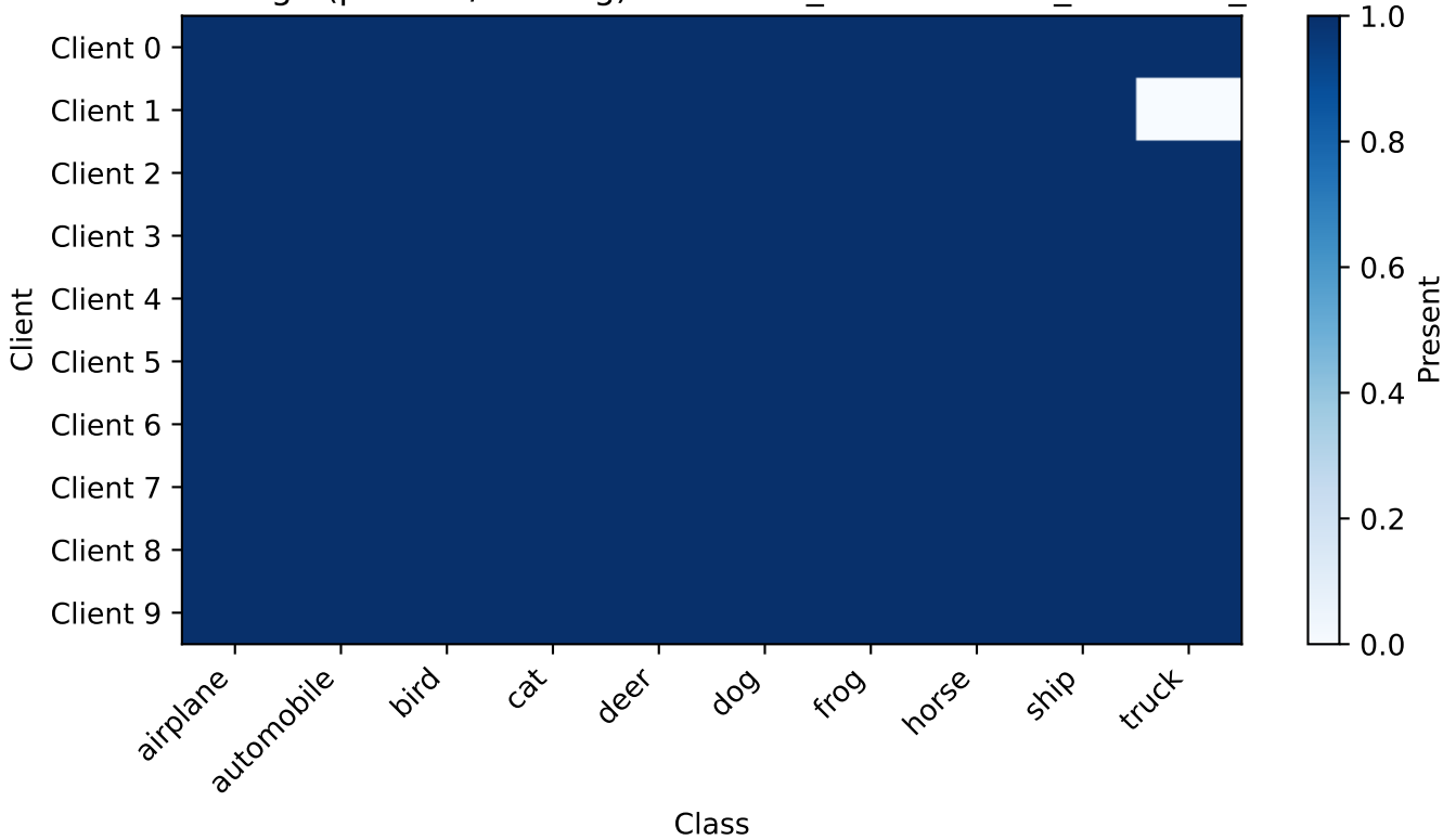
Class coverage (present/missing) — cifar10_dirichlet-a0.5_clients10_seed42
