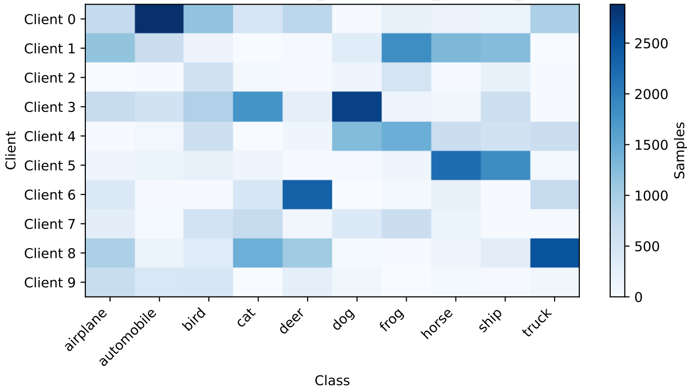
Client class counts — cifar10_dirichlet-a0.5_clients10_seed42
