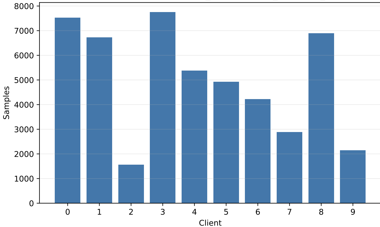
Client partition sizes — cifar10_dirichlet-a0.5_clients10_seed42
