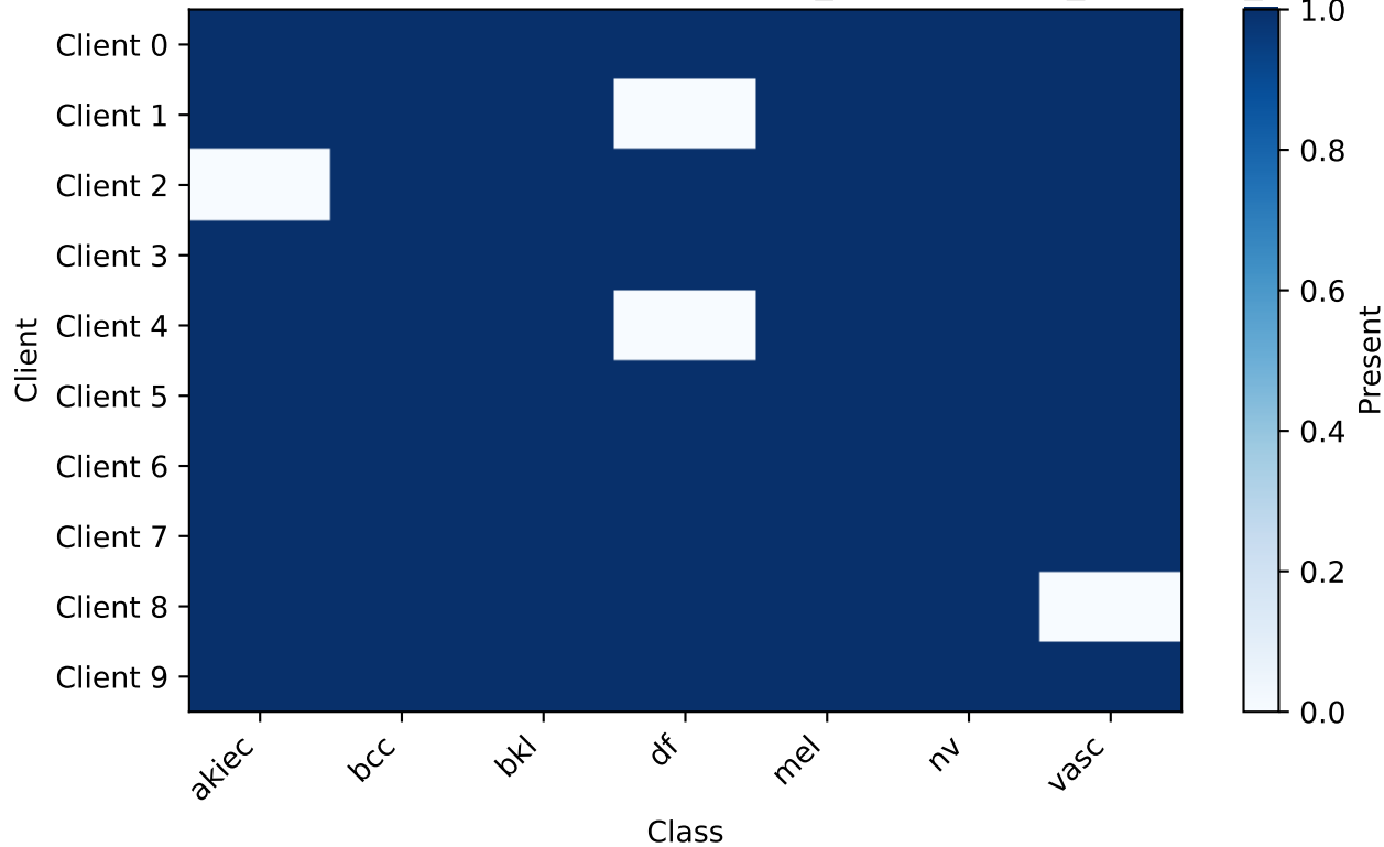
Class coverage (present/missing) — ham10000_dirichlet-a0.5_clients10_seed42
