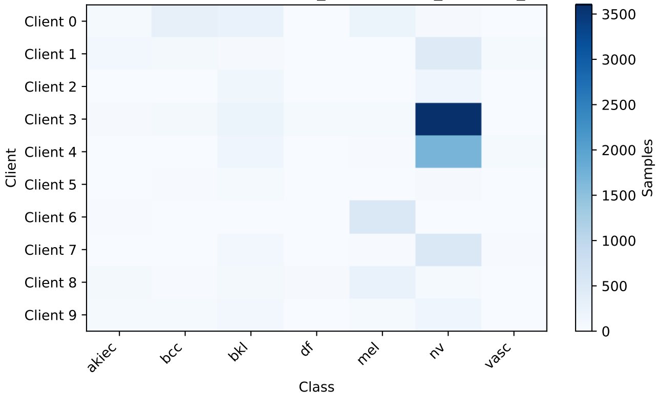
Client class counts — ham10000_dirichlet-a0.5_clients10_seed42
