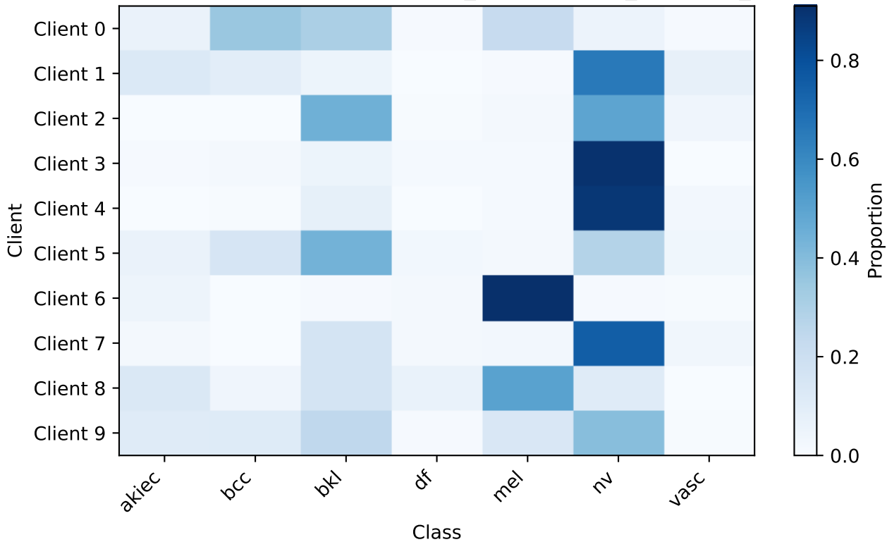
Client class proportions — ham10000_dirichlet-a0.5_clients10_seed42
