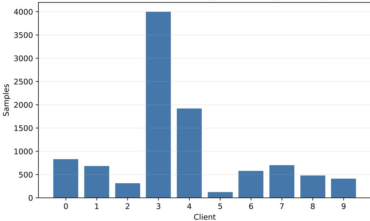
Client partition sizes — ham10000_dirichlet-a0.5_clients10_seed42
