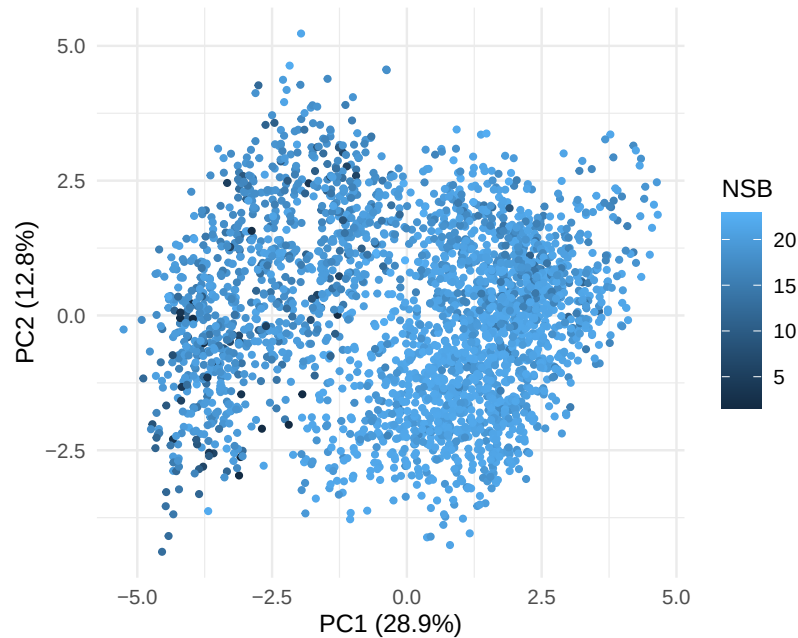
Figure 1: PCA Bi-Plot w/ Night-Sky Brightness Gradient
