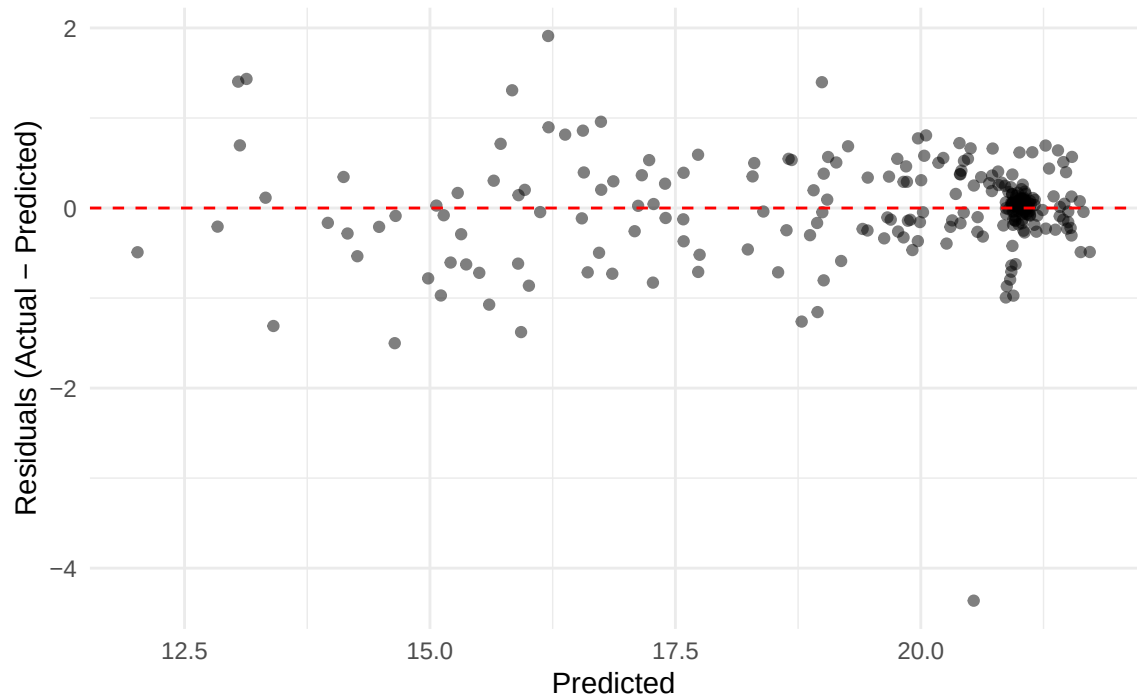
Residuals Plot – BC01
